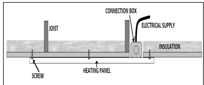
Figure 1 – Surface Mounting
